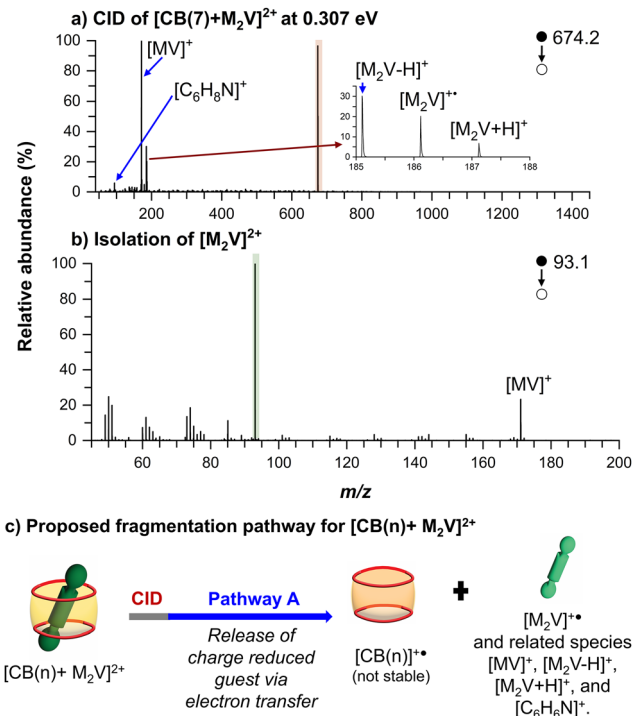
Fig. 1 (a) CID spectrum of [CB(7) + M 2 V] 2+ ( m/z 674.2) at 0.307 eV excitation energy, (b) Fragmentation of [M 2 V] 2+ ( m/z 93.1) during the isolation step in a mass spectrometer (isolation spectra at 0 eV), and (c) scheme showing the proposed fragmentation pathway of [CB(7) + M 2 V] 2+ . In panels a and b precursor m/z are highlighted with colored bars. In panel c the neutral CB host is shown in yellow, while the charged host is shown in orange.
