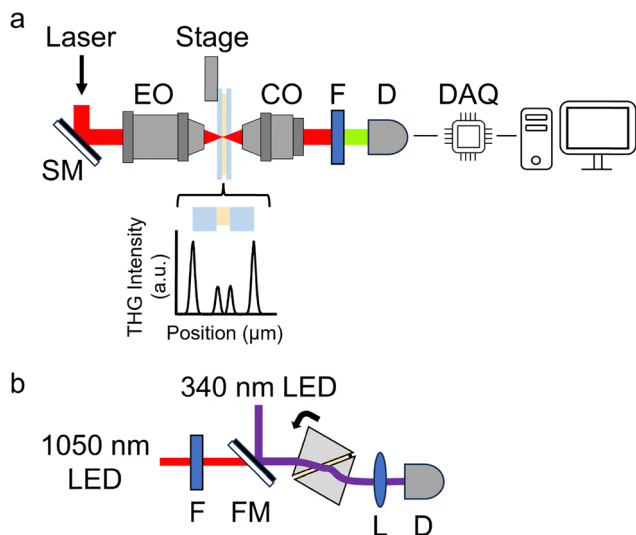
Fig. 2 A schematic of the THG microscope used to collect THG signals at the air–glass and glass–solution interfaces (a) and a schematic of the refractometer (b). The following abbreviations are used in (a): SM – scanning mirrors, EO – excitation objective, CO – collection objective, F – filter, D – detector and DAQ – data acquisition. The following abbreviations are used in (b): F – filter, FM – flipping mirror, L – lens and D – detector.
