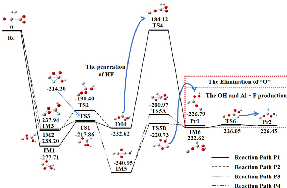
Fig. 8 Potential energy diagram of the Al 2 O 3 /HF system at the B3LYP/6-311+G(3d,2p) level, where the energy is represented in kcal mol -1 .
