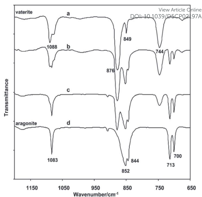
Fig. 8 FTIR spectra (650–1200 cm -1 ) of (a) the vaterite sample, and when it was refluxed in distilled water for (b) 30 min, (c) 60 min, and (d) 75 min. Adapted from reference 27 with permission from American Chemical Society, copyright 2010.
