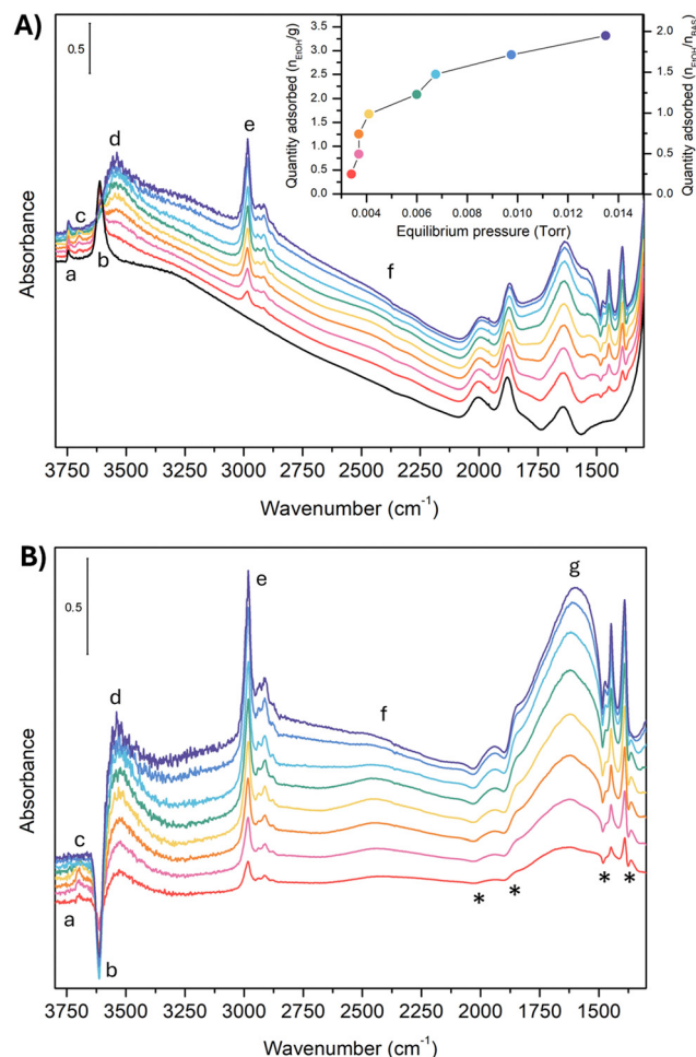
Fig. 1 Experimental IR spectra of unloaded H-ZSM-5 (black line) and H-ZSM-5 loaded with ethanol at increasing pressure (from red to blue). Panel (A) measured adsorbance ( A ). In the inset, the adsorption isotherm. Panel (B) difference spectra at increasing pressure compared to the unloaded zeolite ( A_{\text{diff}} ). The (*) indicate the artificial, derivative-type bands. The spectra are all reported in arbitrary units. No baseline correction has been introduced.
