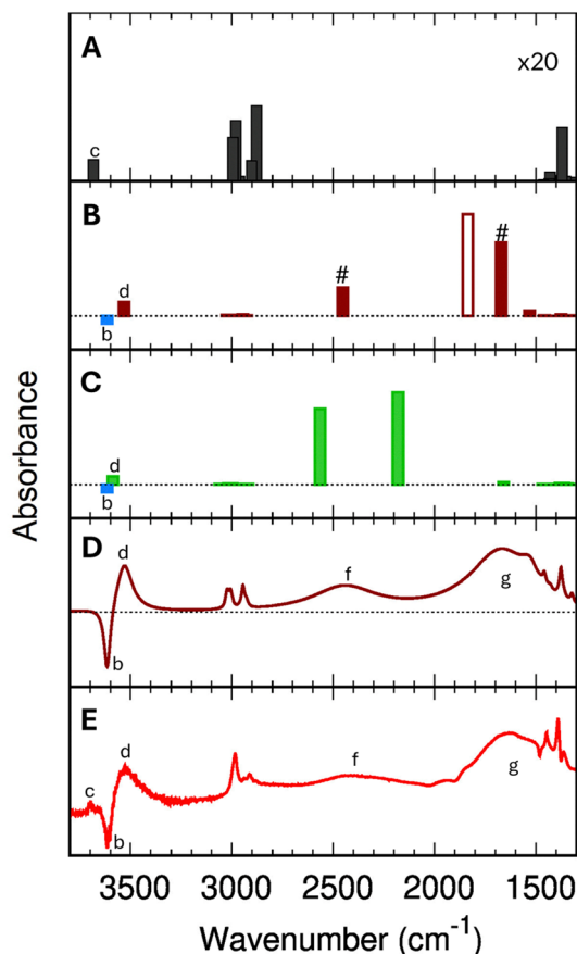
Fig. 5 B3LYP+D2 IR spectra (scaled with 0.9710) for isolated gas-phase ethanol molecules (panel A), intensities multiplied with 20), for single adsorbed ethanol molecules (1 EtOH/BAS, panel B)), and for the protonated adsorbed dimer (2 EtOH/BAS, panel C)). For the single adsorbed ethanol (panel B)), the # indicates the two bands resulting from the Fermi resonance, while the empty bar shows the harmonic (fundamental) (Z)O–H stretching band. The blue bar in panel (B) and (C) marks the position of the (Z)O–H stretching mode of the free BAS (unloaded H-ZSM-5). Panel (D) simulated IR difference spectrum for a single adsorbed ethanol molecule based on B3LYP+D2 results using the Fermi resonance model and assuming a Lorentzian shape with bandwidths given in the ESI,† Section S7. Panel (E) experimental difference spectrum ( A_{\text{diff}} ) at 0.0034 torr (red trace in Fig. 2).
