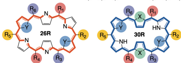
Fig. 1 Graphical representation of the [26]- and [30]hexaphyrins with the X_2Y_2A_2B_2C_2 pattern with three pairs of meso -substitution sites ( \text{R}_{1,4} ; \text{R}_{2,5} ; \text{R}_{3,6} ) and one or two sets of core-modification sites (X, Y). For 26R , only Y modifications were allowed.
