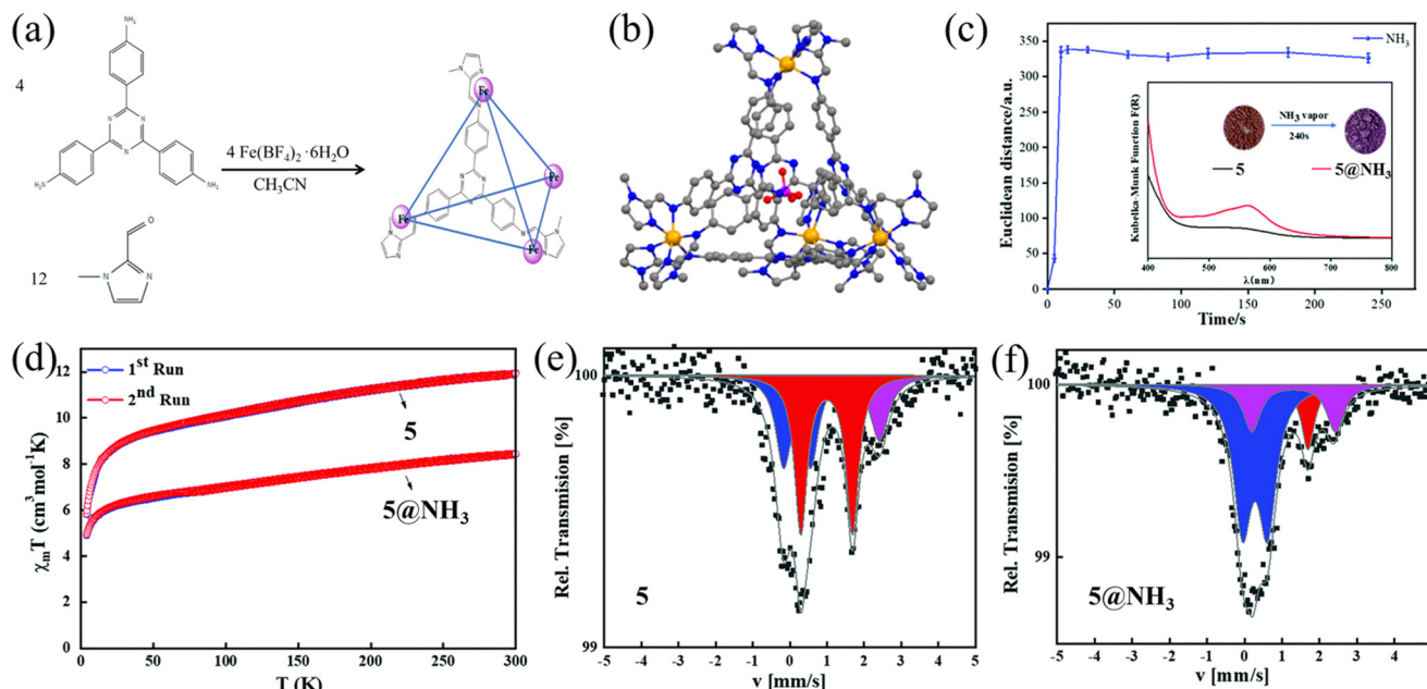
Fig. 7 Synthesis method (a) and crystal structure (b) of 5 . (c) Response time of 5 to \text{NH}_3(\text{g}) at room temperature. Inset: diffuse reflectance spectroscopy and photos of 5 and 5@NH 3 (g) . \chi_m T vs. T plots (d) and ^{57}\text{Fe} Mössbauer spectra for 5 (e) and 5@NH 3 (g) (f). 53
