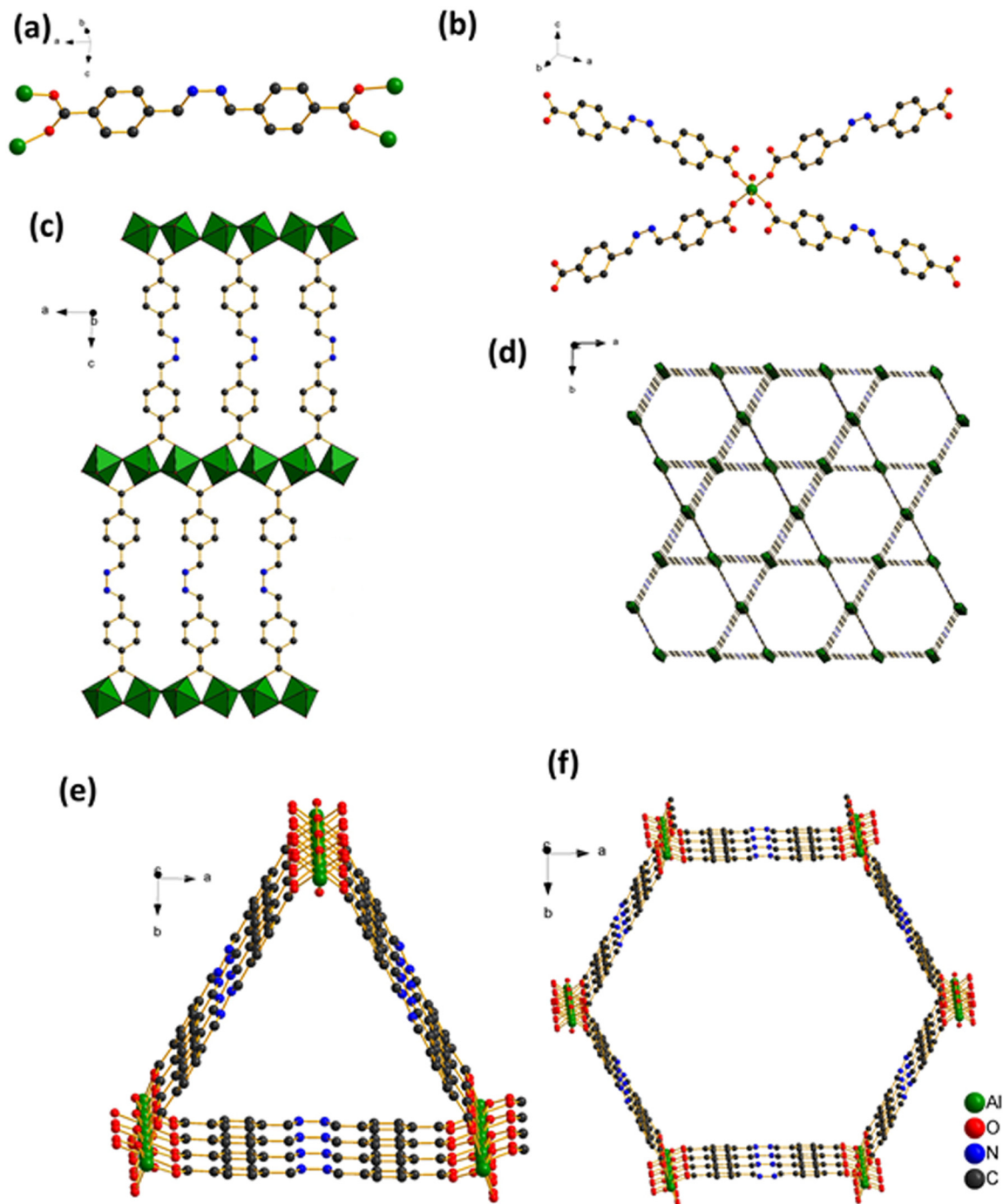
Fig. 1 (a) The coordination environment of the H_2DMDA ligand in the AIDMDA-68. (b) The aluminum ion in AIDMDA-68 is coordinated in an octahedral arrangement. (c) Coordination modes of one-dimensional inorganic chains and their ligands. (d) A 3D structure of AIDMDA-68. (e) Microporous triangular window channels of AIDMDA-68. (f) Mesoporous hexagonal window channels of AIDMDA-68.
