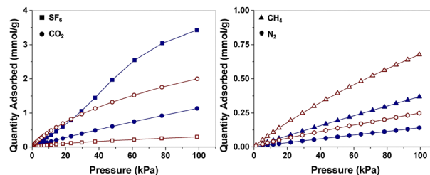
Fig. 4 \text{N}_2 , \text{CH}_4 , \text{SF}_6 and \text{CO}_2 adsorption isotherms of CTH-41 (blue, closed symbols) and CTH-42 (brown, open symbols) recorded at 20 °C.
