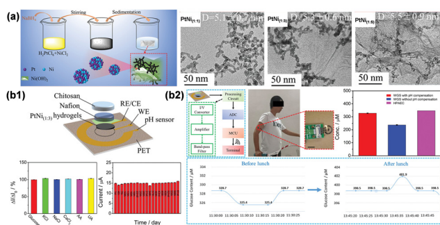
Fig. 7 (a) Synthesis, morphology and structure of the PtNi (1:X) dual aerogels. (b1) Schematic illustration, the selectivity and the long-term stability of the PtNi (1:3) aerogel-based sensing chip. (b2) Wearable application of the PtNi (1:3) dual aerogel-based glucose sensor (copyright 2023, John Wiley and Sons). 85
