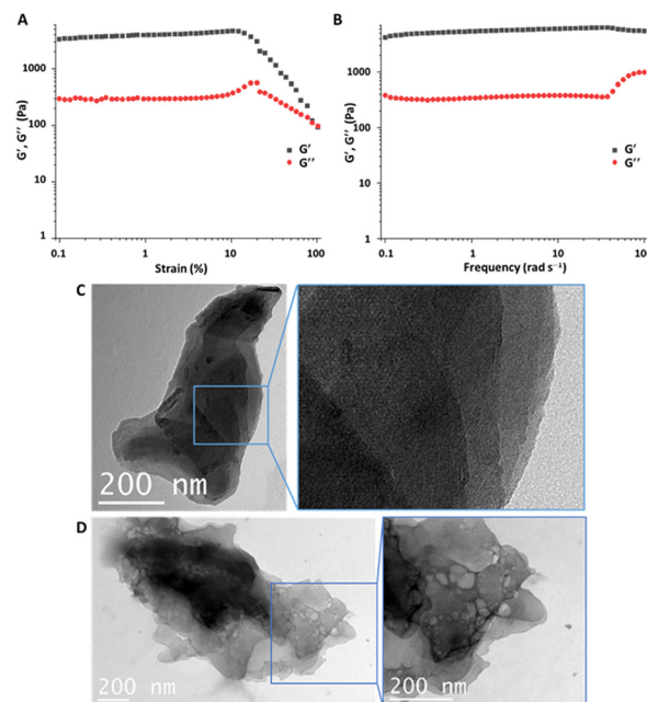
Fig. 3 (A) Strain sweep measurements (at a constant frequency of 1 \text{ rad s}^{-1} ); (B) frequency sweep measurements (at a constant strain of 5%); (C)/(D) HRTEM of metallogel/solution phase nanosheet obtained through \text{Pd}(\text{II}) -directed coordination polymerization of cage 1a (at 15 mM/5 mM conc. of \text{Pd}(\text{II}) ).
