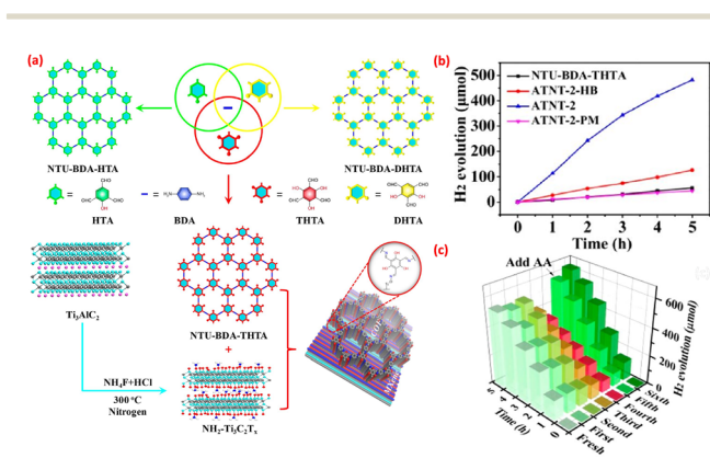
Fig. 12 (a) Synthesis of the COF/MXene- \text{NH}_2 hybrid; (b) photocatalytic activity of synthesized hybrids; and (c) recyclability. Reprinted with permission from ref. 35. Copyright 2020 American Chemical Society.
