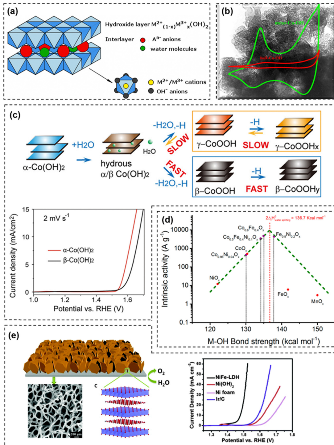
Fig. 5 Base metal hydroxide-based OER electrocatalysts: (a) schematic of layered double hydroxide, 105 (b) cyclic voltammety at 50 \text{ mV s}^{-1} in 1.0 \text{ M KOH} solution of bulk-Co-OH and meso-Co-OH, 106 (c) schematic of the phase transition of Co(OH)_2 in the OER with LSV curves at a scan rate of 2 \text{ mV s}^{-1} after the correction ( iR compensation: 100%), 107 (d) volcano plot of the intrinsic activities of transition metal (oxy)hydroxides vs. M-OH bond strength where the green dotted lines indicate a hypothetical, perfect volcano, 108 and (e) schematic of the NiFe-LDH nanoplate with LSV curves. 109 Reproduced with permissions from ref. 105 and 106, Copyright 2019 and 2016 Elsevier, ref. 107 and 108, Copyright 2022 and 2016 American Chemical Society and ref. 109, Copyright 2014 Royal Society of Chemistry.
