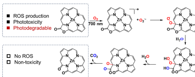
Fig. 7 Schematic illustration of conversion from ZnBPL to ZnBPD. Figure adapted from ref. 29 Copyright: 2022, with the permission from John Wiley and Sons.
