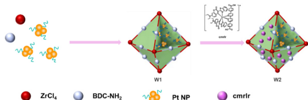
Fig. 1 Scheme for the preparation of cmrIr/Pt@UiO-66-NH 2 .
