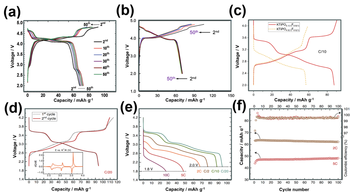
Fig. 14 Voltage-capacity profiles of (a) KVPO 4 ( \alpha -polymorph) and (b) KVPO 4 F. The theoretical capacity of KVPO 4 and KVPO 4 F is 133.3 mA h g -1 and 131.4 mA h g -1 , respectively. (c) Voltage profile comparisons of KTiPO 4 F and KTiPO 4.5 F 0.5 . (d) Voltage profiles of KTiPO 4 F at C/20 rate, (e) corresponding rate performance and (f) cycle performance at various current densities. The theoretical capacity of KTiPO 4 F and KTiPO 4.5 F 0.5 is 133.4 mA h g -1 and 134.4 mA h g -1 , respectively. Figures (a) and (b) reproduced from ref. 18 with permission. Copyright 2017 Royal Society of Chemistry. Figures (c), (d)–(f) reproduced with permission from ref. 180. Copyright 2020 Springer Nature.
