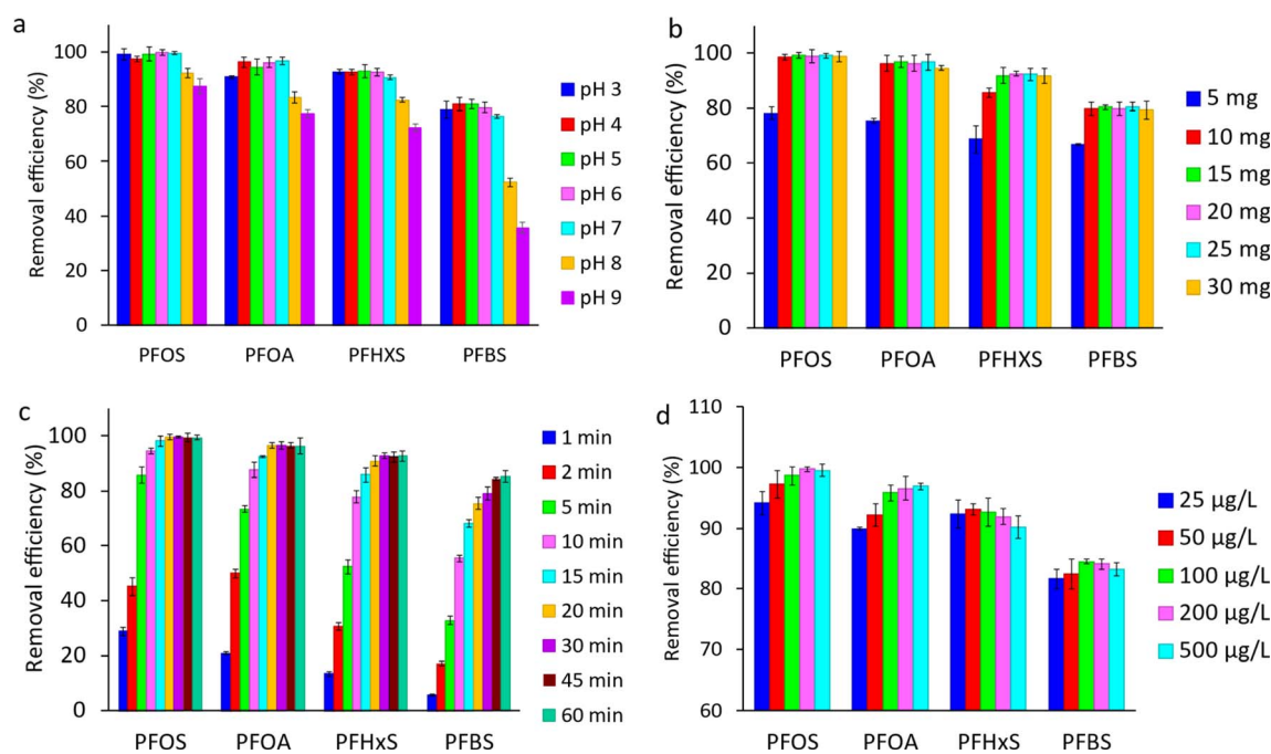
Fig. 9 (a) Effect of the solution pH on PFAS removal efficiency (conditions: 40 mL of 500 \mu\text{g L}^{-1} PFAS, 20 mg adsorbent, and 30 min extraction time); (b) effect of adsorbent amount on PFAS removal efficiency (conditions: 40 mL of 500 \mu\text{g L}^{-1} PFAS, pH 6.5, and 30 min extraction time); (c) effect of contact time on the removal efficiency of PFAS (conditions: 40 mL of 500 \mu\text{g L}^{-1} PFAS, pH 6.5, and 15 mg adsorbent); and (d) effect of initial PFAS concentration on the removal efficiency (conditions: 40 mL PFAS solution, pH 6.5, 15 mg adsorbent, and 30 min extraction time).
