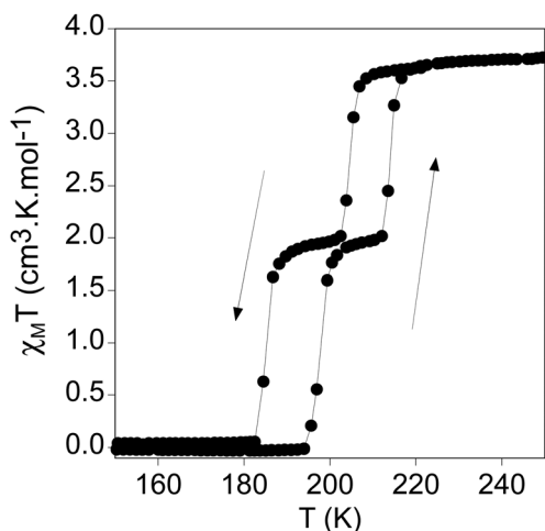
Fig. 2 \chi_M T vs. temperature of 1 in contact with the mother liquor.
