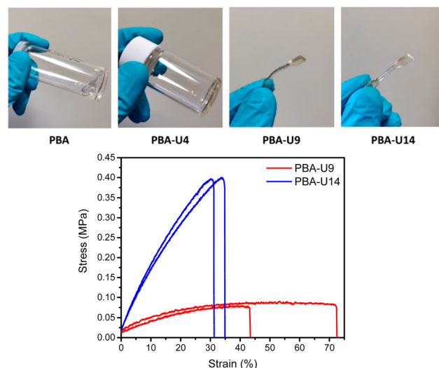
Fig. 13 Top: Physical appearance of the PBA polymer compared to PBA-UPy materials; PBA-U4 still showed viscous liquid behavior, while PBA-U9 and PBA-U14 could be compression molded and pressed into dog bones for tensile testing. Bottom: Tensile test stress-strain curves of PBA-U9 and PBA-U14.
