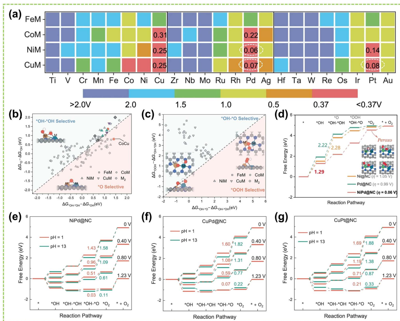
Fig. 19 The OER performance of DACs in all pH conditions. (a) Activity map. The computed overpotential of the FeM, CoM, NiM, and CuM dimers on M'M@NC. (b) \Delta G of \text{*OH} toward \text{*OH-*OH} versus \text{*OH} \rightarrow \text{*O} + \text{H}^+ + \text{e}^- . Data points screened for high-performance homo- and hetero-nuclear catalysts are colored. (c) \Delta G of \text{*OH-*OH} \rightarrow \text{*OH-*O} + \text{H}^+ + \text{e}^- versus \text{*OH-*OH} \rightarrow \text{*OOH} + \text{H}^+ + \text{e}^- . Insets: the schematic configuration of the different intermediates adsorbed on M'M@NC. The white, red, gray, and blue spheres in the atomic models represent H, O, C, and N atoms, respectively. (d) Free energy diagrams of NiPd@NC and the respective corresponding SACs for OER. Inset: the optimized configurations of oxygenated intermediates represented as NiPd@NC. Free energy diagrams of (e) NiPd@NC, (f) CuPd@NC, and (g) CuPt@NC at different potentials with pH = 1 and 13 and the corresponding \Delta G_{\text{*OH-*O} \rightarrow \text{*O}_2} are labeled 89 (reproduced with permission from ref. 89 copyright 2023, Springer Nature).
