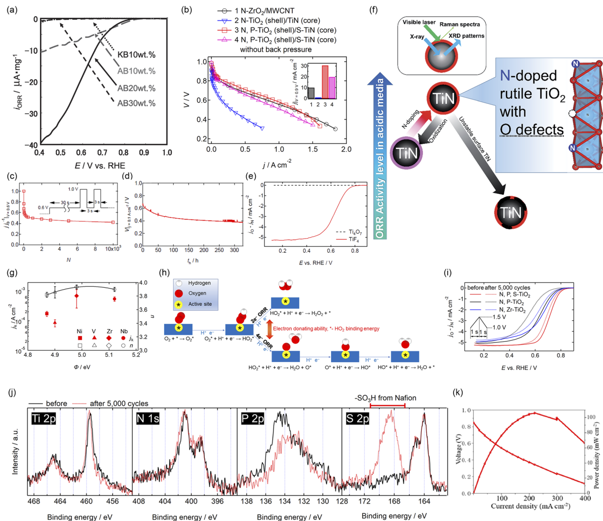
Fig. 12 (a) ORR mass activity versus potential ( i_{\text{ORR}} - E ) curves of a \text{ZrO}_2 catalyst for four different catalyst layers in 0.1 \text{mol dm}^{-3} \text{H}_2\text{SO}_4 without rotation. The catalyst layers were formed by mixing the \text{ZrO}_2 catalyst with two different carbon black materials, Ketjen Black EC300J (KB) or acetylene black (AB). The mass fraction of KB was set constant at 10% w/w, whereas that of AB was set at 10, 20, and 30% w/w. Reproduced with permission. 222 Copyright 2011, The Electrochemical Society of Japan. (b) V - j curves of MEAs for three different catalysts at the cathode, (1) N- \text{ZrO}_2/\text{MWCNT} , (2) N- \text{TiO}_2 (shell)/TiN (core), and (3) N, P- \text{TiO}_2 (shell)/S-TiN (core) at 353 K. The cathode catalyst loadings, m , were 10, 4.7, and 5.8 \text{mg cm}^{-2} , respectively, for MEAs 1, 2, and 3. In all MEAs, the anode was commercial 46% w/w Pt/C with 0.3 \text{mg}_{\text{Pt}} \text{cm}^{-2} Pt loading. The anode and cathode were supplied with fully humidified \text{H}_2 with 0.2 MPa (gauge) and \text{O}_2 with 0.3 MPa (gauge) back pressures, respectively. MEA 3 was also operated without back pressure at the anode and cathode, and is labeled as 4. The inset shows j at V = 0.9 \text{ V} from the four curves. Reproduced with permission. 38,223 Copyright 2016, Elsevier, Copyright 2017, American Chemical Society. (c) A normalized j at V = 0.6 \text{ V} versus FCCJ load cycle number ( j_{0.6 \text{ V}}^{-1} / \text{V} - N ) curve and (d) a cell voltage versus time held at 0.1 \text{A cm}^{-2} ( V_{j=0.1 \text{ A cm}^{-2}} - t_{\text{h}} ) curves of MEAs with the N- \text{ZrO}_2/\text{MWCNT} cathode catalyst. m was 8.3 and 8.9 \text{mg cm}^{-2} for (c) and (d), respectively. Reproduced with permission. 223 Copyright 2017, American Chemical Society. (e) RDE voltammograms of two N- \text{TiO}_2 catalysts synthesized by mixing urea and one of the two titanium sources, \text{Ti}_4\text{O}_7 and \text{TiF}_4 , in 1.0 \text{mol dm}^{-3} HCl solution, followed by pyrolysis at 1123 K. The scans were performed under \text{N}_2 and \text{O}_2 atmospheres, with a rotation speed of 1500 rpm and a scan rate of -5 \text{ mV s}^{-1} (cathodic) in 0.1 \text{mol dm}^{-3} \text{H}_2\text{SO}_4 . Reproduced with permission. 224 Copyright 2018, American Chemical Society. (f) A schematic image of N- \text{TiO}_2 catalysts and the ORR active site. Reproduced with permission. 225 Copyright 2016, Royal Society of Chemistry. (g) Kinetic current density and number of electrons transferred per unit \text{O}_2 molecule versus the work function curves ( j_{\text{k}} - \Phi and n - \Phi curves, respectively) derived from the RDE voltammograms of four N, M- \text{TiO}_2/\text{S-TiN} catalysts, where M = Zr, Nb, Ni, and V. (h) Two reaction pathways for the ORR on conventional catalysts. Reproduced with permission. 226 Copyright 2022, Royal Society of Chemistry. (i) RDE voltammograms of N, P- \text{TiO}_2/\text{S-TiN} , N, Zr- \text{TiO}_2/\text{S-TiN} , and N, P, S- \text{TiO}_2/\text{S-TiN} catalysts before (solid curves) and after (dashed curves) 5000 FCCJ startup/shutdown cycles; the protocol is shown in the inset. Reproduced with permission. 227-229 Copyright 2020, American Chemical Society, Copyright 2022, American Chemical Society, Copyright 2024, Royal Society of Chemistry. (j) X-ray photoelectron spectra of the N, P, S- \text{TiO}_2/\text{S-TiN} catalyst before (solid curves) and after (dashed curves) 5000 FCCJ startup/shutdown cycles. The N, P, S- \text{TiO}_2/\text{S-TiN} catalyst after 5000 cycles contains Nafion PFSI in the catalyst layer. Reproduced with permission. 229 Copyright 2024, Royal Society of Chemistry. (k) Cell voltage and power density versus current density curves of an MEA fabricated using \text{Ti}_{0.8}\text{Co}_{0.2}\text{N} at m = 4 \text{ mg cm}^{-2} and commercial 60% w/w Pt/C catalysts at 0.1 \text{mg}_{\text{Pt}} \text{cm}^{-2} in the cathode and anode, respectively, at 343 K. The anode and cathode were supplied with fully humidified \text{H}_2 and air, respectively. Reproduced with permission. 230 Copyright 2018, American Chemical Society.
