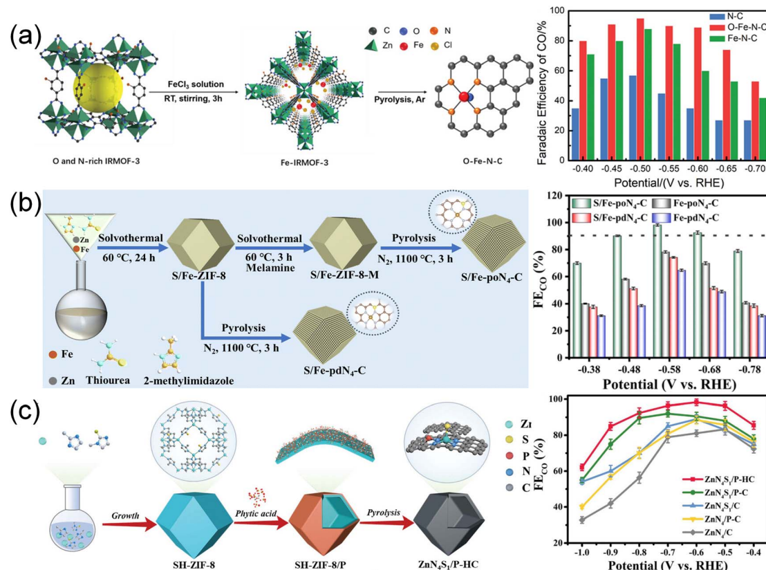
Fig. 11 (a) Schematic synthesis of O-Fe-N-C and \text{FE}_{\text{CO}} in \text{CO}_2 -saturated 0.5 M \text{KHCO}_3 . Copyright 2022, Wiley-VCH. 54 (b) Schematic illustration of preparing S/Fe-po \text{N}_4 -C. Copyright 2024, Royal Society of Chemistry. 88 (c) Schematic illustration of the synthesis of \text{ZnN}_4\text{S}_1/\text{P-HC} . Copyright 2023, Wiley-VCH. 96
