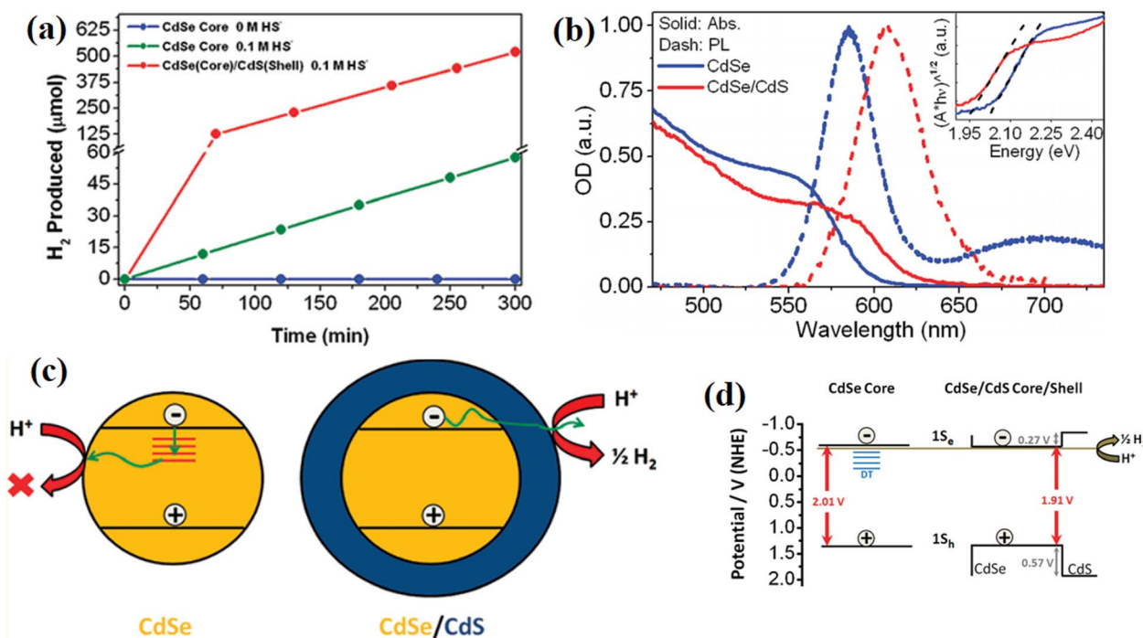
Fig. 21 (a) Photocatalytic hydrogen evolution for CdSe and CdSe/CdS QDs in pure H_2O and 0.1 M HS solution under visible light illumination from a 300 W Xe lamp equipped with a 400 nm long pass filter. (b) Static absorption (solid lines) and photoluminescence (dashed lines) spectra of CdSe (blue lines) and CdSe/CdS core/shell QDs (red lines). (c) and (d) Mechanisms of CdS in passivating the trap states of CdSe and facilitating H_2 evolution. Reproduced with permission from ref. 101. Copyright 2011, the American Chemical Society.
