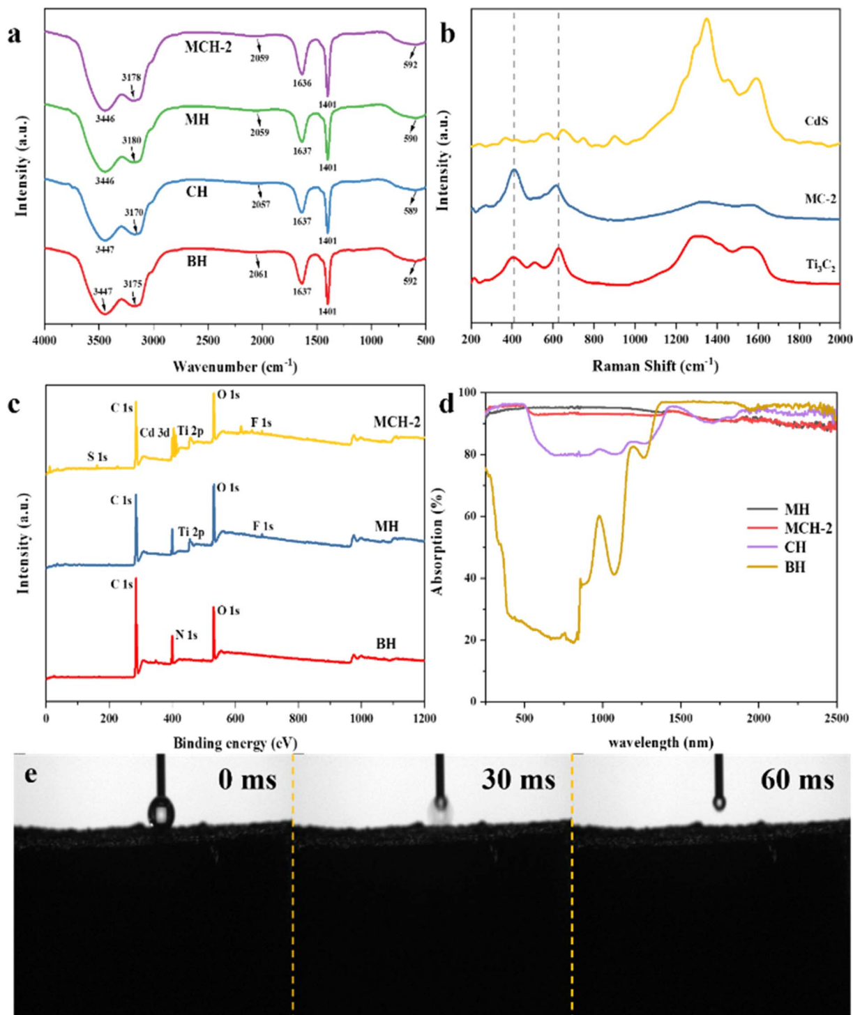
Fig. 4 (a) FTIR spectra of BH, CH, MH, and MCH-2. (b) Raman spectroscopy of \text{Ti}_3\text{C}_2 , MC-2, and CdS. (c) XPS spectra of BH, MH, and MCH-2. (d) UV-vis-NIR absorption spectra of hydrogels. (e) Surface contact angle of MCH-2.
