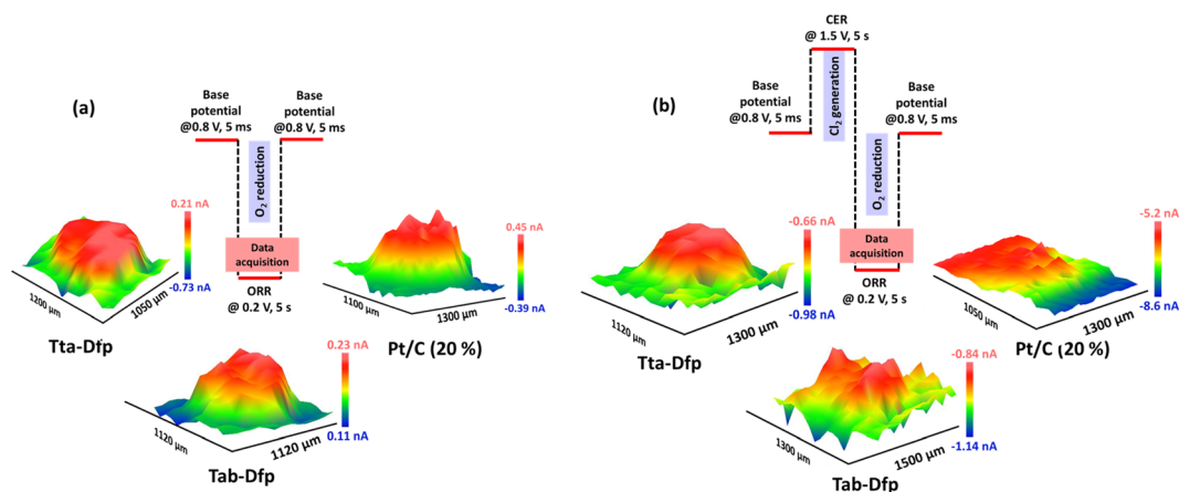
Fig. 5 Potential pulse profile for (a) only the ORR and (b) Cl 2 generation followed by the ORR at the Pt-tip and the corresponding 3D RC-SECM images of Tta-Dfp, Tab-Dfp and Pt/C (20%) measured in 400 mM HCl.
