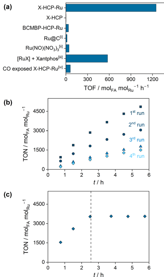
Fig. 2 (a) Catalytic evaluation of X-HCP-Ru and reference experiments for the CO 2 hydrogenation to formic acid. (b) Catalytic recycling of X-HCP-Ru over four recycling steps. Kinetic curves of the 1 st run (squares), 2 nd run (circles), 3 rd run (triangles) and 4 th run (diamonds). (c) Hot leaching experiments of X-HCP-Ru. The catalyst was filtered off after 2.5 h, the remaining filtrate was pressurized and heated up to initial reaction conditions. Reaction conditions: 300 mL Hastelloy autoclave, V(H 2 O) = 150 mL, n (NaHCO 3 ) = 150 mmol, m (cat.) = 200 mg, p (CO 2 /H 2 ) = 60 bar (1 : 1), T = 110 °C, t = 5.5 h, 700 rpm. [i] m (Ru@C) = 50 mg (5 wt%) [ii] n (Ru(NO)(NO 3 ) 3 ) = 15 μmol [iii] V(DMSO) = 150 mL, n (NEt 3 ) = 150 mmol, n ([Ru( p -cymene)Cl 2 ) 2 ) = 0.5 μmol, n (Xantphos) = 0.5 μmol. [iv] Exposure of X-HCP-Ru to CO (5 bar), which is released from the autoclave before the catalysis.
