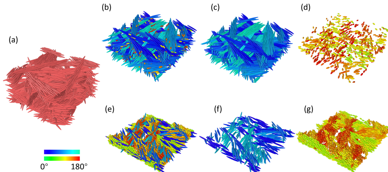
Fig. 7 Structure of co-assemblies: (a) pure CNCs, (b) CNCs : AuNRs: 10 : 1 and (c) 1 : 2. (d), (f) and (g) represent the separated structure of CNCs and AuNRs respectively. The colour coding represents the angle between the elongation direction of the particles and the backplane.
