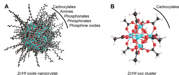
Scheme 1 (A) Schematic representation of a colloidally stable zirconium/hafnium oxide nanocrystal depicting the inorganic core and organic ligand shell. (B) The structure of M_6O_8H_4(OOCR)_{12} , where the M_6O_8 core is capped with four protons and twelve carboxylate ligands, M = \text{Zr}/\text{Hf} . The ligands that have been reported to cap nanocrystals and clusters in nonpolar media are listed. Cyan atoms represent zirconium or hafnium, all other atoms follow conventional CPK coloring.
