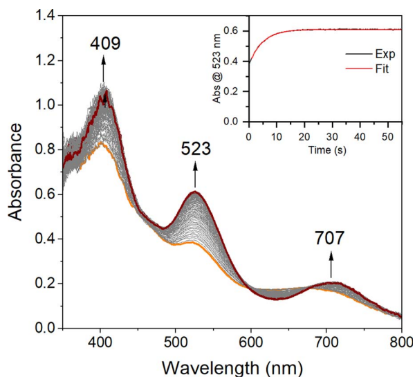
Fig. 5 Time-resolved spectral changes observed in the reaction between 3 (0.1 mM) and KO 2 (5.0 mM; solubilized with 222-KryptoFix) in THF at -40 °C. Inset: kinetic trace ( \lambda = 523 nm) showing the formation of 2 . All reported concentrations are after mixing in the stopped-flow cell.
