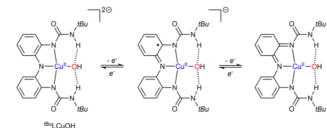
Scheme 9 Characterized oxidation states reached via reduction/oxidation of ^tBuLCuOH . Adapted from ref. 73.
