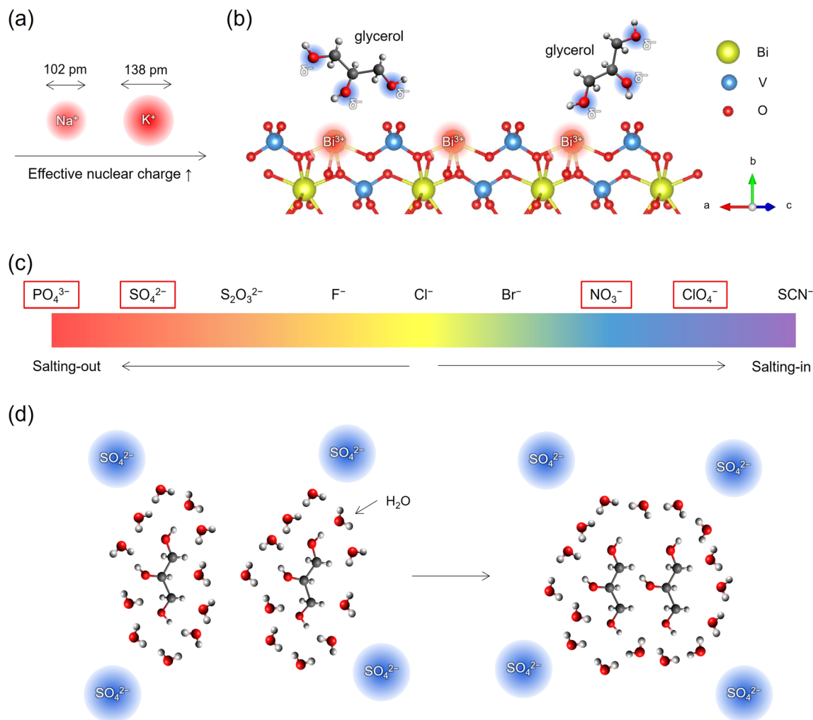
Fig. 5 Schematic illustrations of (a) Na + and K + ions with distinct effective ionic radii, leading to varying effective nuclear charges, and (b) the BiVO 4 surface interaction with glycerol: hydroxyls of glycerol, carrying a partial negative charge (δ - ), are electrostatically drawn to the Bi 3+ ions on the BiVO 4 surface. (c) The Hofmeister series. (d) Schematic illustration of the aggregation of glycerol molecules induced by the presence of SO 4 2- anions.
