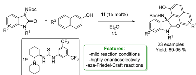
Scheme 43 Takemoto-type organocatalyst catalyzed aza-Friedel-Crafts addition of naphthols with isatin-derived ketimines. 131
