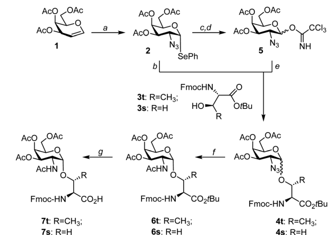
Scheme 1 Synthesis of Fmoc-Thr( \alpha Ac 3 GalNAc)-OH and Fmoc-Ser( \alpha Ac 3 GalNAc)-OH. Conditions: (a) \text{Se}_2\text{Ph}_2 , trimethylsilyl azide, \text{PhI}(\text{OAc})_2 , \text{CH}_2\text{Cl}_2 , -30^\circ\text{C} (55%); (b) N -iodosuccinimide, trimethylsilyl triflate, \text{CH}_2\text{Cl}_2 , \text{Et}_2\text{O} , 0^\circ\text{C} ; (c) N -iodosuccinimide, acetone, \text{H}_2\text{O} , RT (quant.); (d) \text{CCl}_3\text{CN} , \text{Cs}_2\text{CO}_3 , \text{CH}_2\text{Cl}_2 , RT (84%); (e) trimethylsilyl triflate, \text{CH}_2\text{Cl}_2 , \text{Et}_2\text{O} , 0^\circ\text{C} ; (f) \text{Zn} , THF, AcOH, Ac 2 O, RT; (g) TFA, \text{CH}_2\text{Cl}_2 , RT (70–75%).
