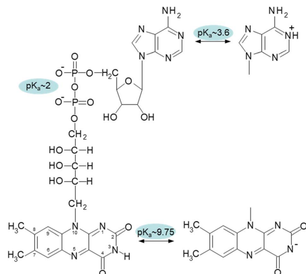
Fig. 1 Chemical structure of oxidized form of FAD with designated pK a values of the corresponding groups: N-1 of adenine with pK a ~ 3.6, diphosphate with pK a ~ 2, and N-3 of isoalloxazine ring with pK a ~ 9.75.
