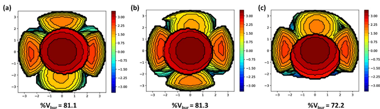
Fig. 4 Steric maps of 1 (a), 2 (b) and 3 (c) with % V_{\text{bur}} generated using SambVca 2.1 web application.
