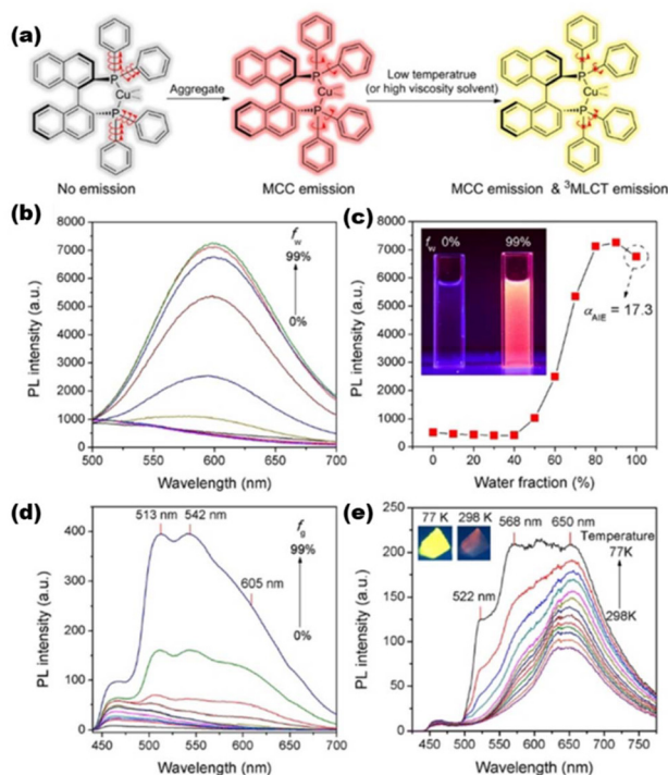
Fig. 3 (a) RIM mechanism of the \text{R/S-Cu}_3 nanocluster; (b) emission spectra of \text{R/S-Cu}_3 in DMSO-H 2 O mixtures with different ratios; (c) emission intensity of \text{R/S-Cu}_3 at 605 nm as a function of the volume fraction of water ( f_w ); (d) emission spectra of \text{R/S-Cu}_3 in EtOH-glycerol mixtures with different f_g values; and (e) temperature-dependent emission spectra of \text{R/S-Cu}_3 in the solid state. Reproduced from ref. 99 with permission from Wiley, copyright (2020).
