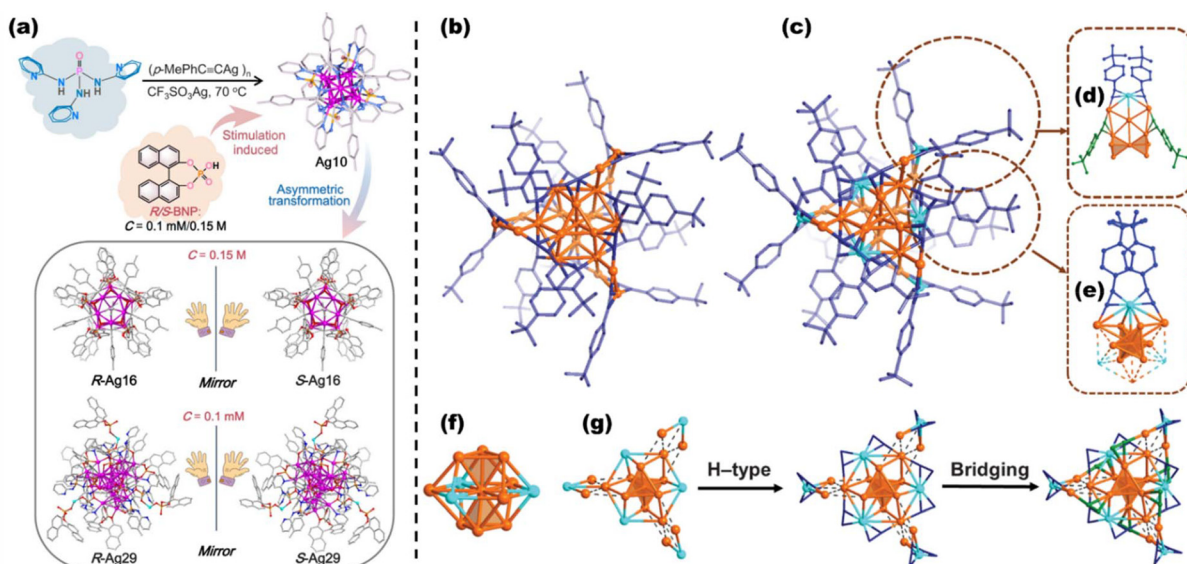
Fig. 7 (a) Varying amounts of R/S\text{-BNP} ligands bring about the asymmetric transformation of achiral \text{Ag}_{10} to chiral R/\text{S-Ag}_{16} and R/\text{S-Ag}_{29} . Reproduced from ref. 155 with permission from the American Chemical Society, copyright (2024). Topological structures of \text{Au}_{22} (b) and \text{Au}_{16}\text{Cu}_6 (c) nanoclusters, H atoms are omitted for clarity. Coordination modes of Cu atoms in the \text{Au}_2\text{Cu} motifs (d) and \text{Au}_6\text{Cu}_6 motifs of \text{Au}_{16}\text{Cu}_6 . (f) \text{Au}_{10}\text{Cu}_3 kernel of \text{Au}_{16}\text{Cu}_6 . (g) Structural evolution of \text{Au}_{16}\text{Cu}_6 , tert -butyl phenyl groups are omitted for clarity. Note: Au = orange; Cu = light blue; C = blue/deep blue/or green. Reproduced from ref. 164 with permission from the American Association for the Advancement of Science, copyright (2024).
