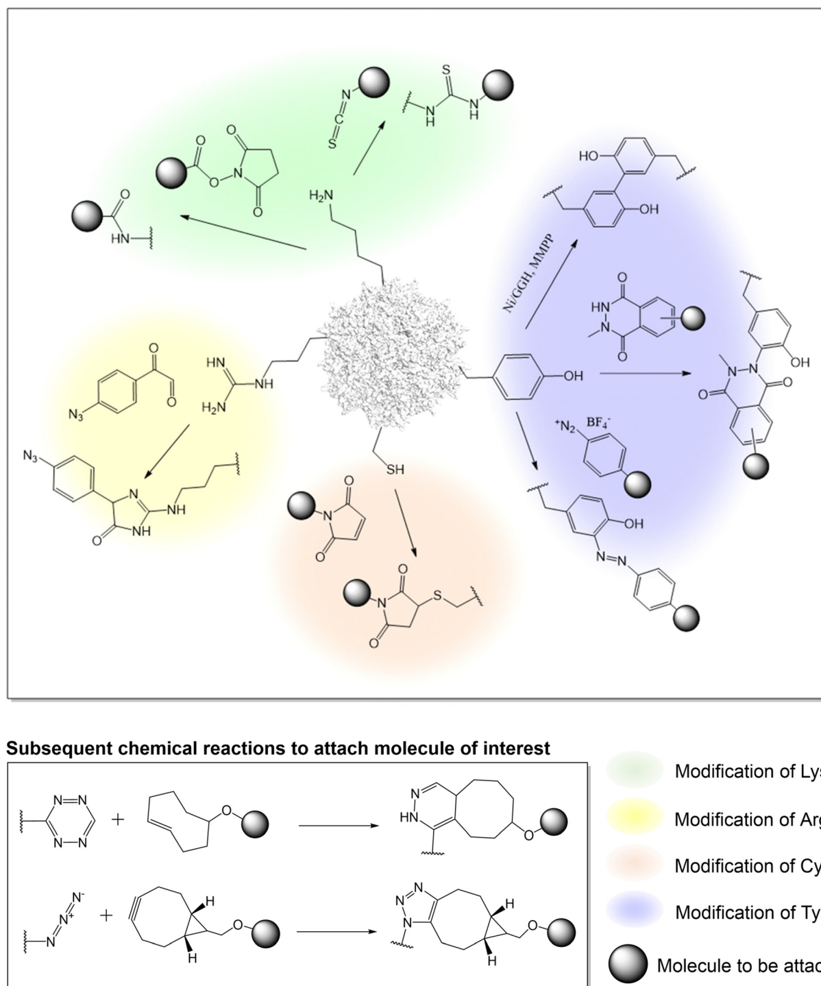
Fig. 1 Various chemistry on canonical amino acids to engineer the AAV capsid.
