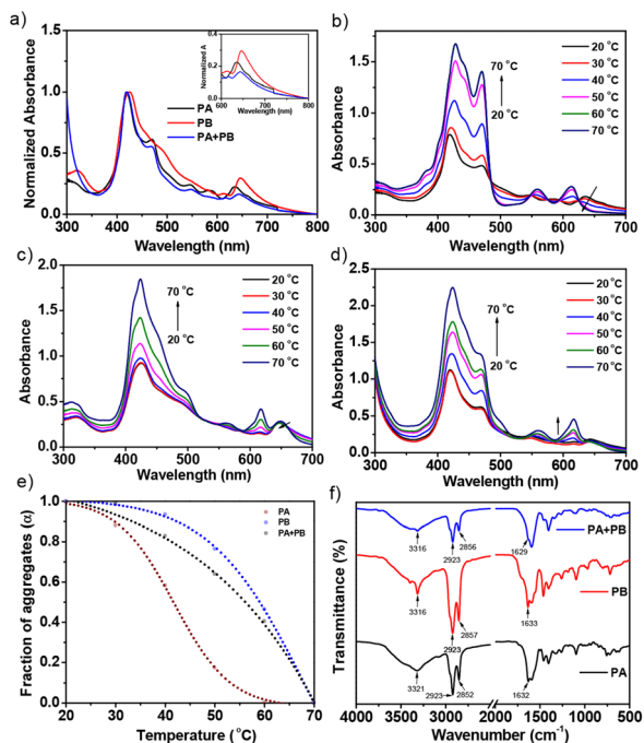
Fig. 2 (a) Normalized ultraviolet–visible absorption spectra of PA , PB , and PA + PB (1 : 1 M) in cyclohexane at a concentration of 1 \times 10^{-5} M at 25 °C. The inset shows the conspicuous UV-shift in the peaks of PA , PB , and PA + PB . (b–d) Temperature-dependent UV–visible absorption spectra of PA , PB and PA + PB assemblies in cyclohexane with an increment in temperature from 20 °C to 70 °C. (e) Fraction of aggregates ( \alpha_{\text{agg}} ) of PA , PB and PA + PB calculated from apparent absorption intensity at the Soret band: \lambda = 420 nm at different temperatures. (f) FT-IR analysis of PA , PB and PA + PB aggregates denoting the considerable stretching frequencies of N–H, C–H, C=O and N–H bending frequencies.
