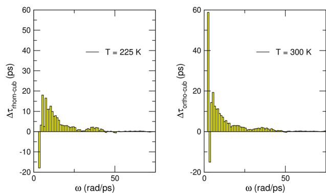
Fig. 6 Phonon lifetimes of the polar and nonpolar phases of KNO expressed as a function of phonon frequency. \Delta\tau_{x\text{-cub}} \equiv \tau_x - \tau_{\text{cub}} results are averaged over frequency intervals of 1 \text{ rad ps}^{-1} and correspond to R3m \rightarrow Pm\bar{3}m at 225 K and Amm2 \rightarrow Pm\bar{3}m at 300 K.
