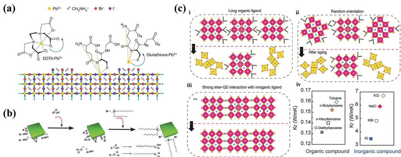
Fig. 11 (a) Schematic diagram of the interactions of GSH and EDTA with Pb^{2+} atoms on the NCs surface. Reproduced with permission from ref. 193. Copyright 2021 Springer Nature. (b) The ligand-exchange mechanism on CsPbBr_3 NC surfaces treated sequentially by OA and DDAB. Reproduced with permission from ref. 199. Copyright 2016 Wiley-VCH. (c) Formation of strained films with increased thermal transport. Reproduced with permission from ref. 201. Copyright 2021 Wiley-VCH.
