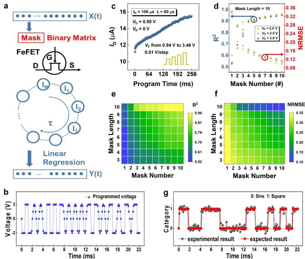
Fig. 5 Waveform classification realized with dynamic RC system. (a) Schematic of the dynamic RC system demonstrated on integrated \text{MoS}_2\text{-H}_2\text{O} based FeFETs. Before a given input vector is transformed into the system, a binary mask containing '–1' and '1' elements were used to process the signal to increase the number of virtual nodes. The entire response under the mask occurs within a duration time \tau . Linear regression model is used to get the weights ( W_{out} ) and the output vector is a linear combination of the virtual nodes. (b) The input sequence was a random combination of sine and square waveforms and transferred into the devices by discrete voltage. (c) The modulation of conductance states with the pulse train demonstrates the device's capability to respond to a series of non-identical amplitude pulse trains. Non-identical programming bias ( V_p ) was introduced from 0.94 V to 3.46 V at 0.01 V per step. The fixed programming time ( t_p ) of 100 \mu s was applied to all the input pulse trains, with an interval time ( t_i ) of 60 \mu s . The read voltage ( V_{read} ) of 0 V with V_D = 0.5 V was set to measure the post-synaptic conductance. (d) Variation of R^2 and NRMSE as a function of the number of paralleled reservoirs under different programmed voltage. The contour maps show variation of (e) R^2 and (f) NRMSE with respect to mask number and mask length. (g) The classification results of waveforms were obtained using 10 masks, each with a mask length set to 10. The desired output was a binary sequence consisting of '0' and '1', representing sine and square waveforms, respectively.
