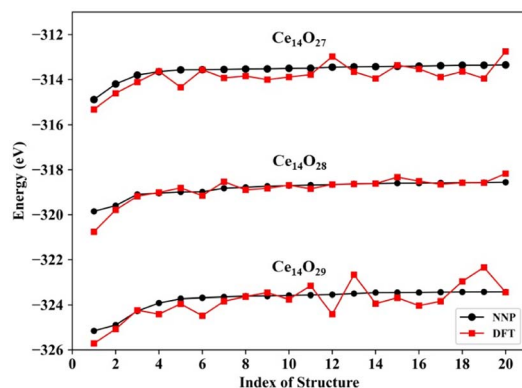
Fig. 3 Comparison of the NNP and DFT energies of the top 20 low-energy structures of the Ce_{14}O_x ( x = 27, 28 , and 29 ) structures (NNP: energies by neural network potential prediction, DFT: energies by DFT calculation).
