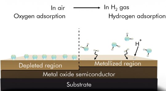
Fig. 4 \text{H}_2 sensing mechanisms of MOx based \text{H}_2 sensors. (a) Reducing gas effect. (b) Metallization effect; reprinted (adapted) with permission from ref. 43. Copyright 2020 American Chemical Society.
