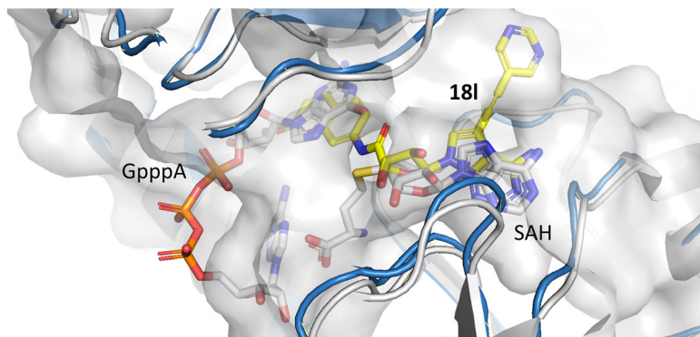
Fig. 3 Correlation between IC_{50} values and GlideScore XP (left). Docking pose of 18l in nsp14 (PDB: 7R2V; 35 protein in blue, inhibitor in yellow) overlaid with nsp14 with a cap analog (GpppA, gray) and SAH (PDB: 5C8S; 40 gray) (right).
