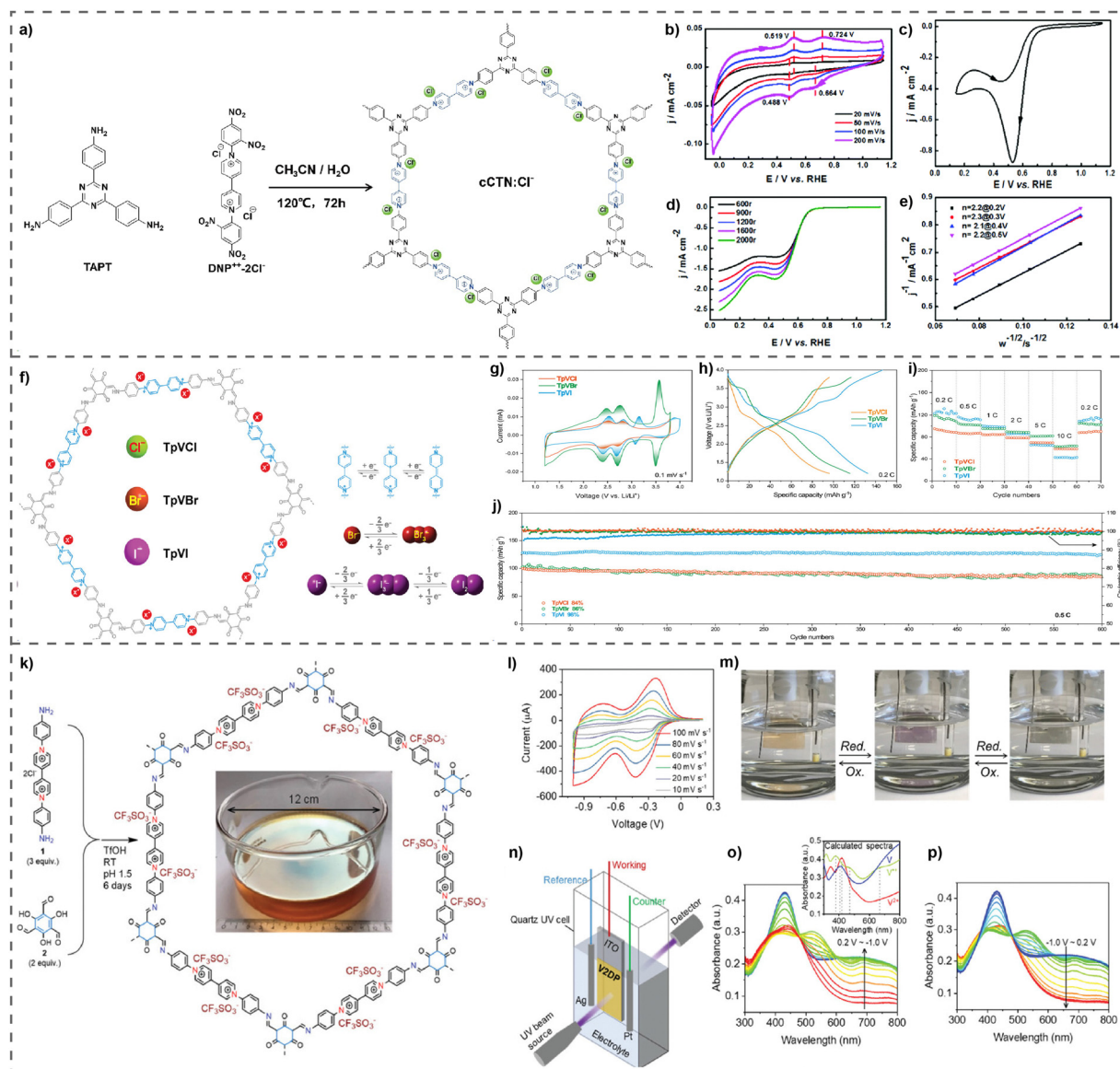
Fig. 9 (a) Synthesis of \text{cCTN:Cl}^- , (b) CVs of \text{cCTN:Cl}^- , (c) CV of \text{cCTN:Cl}^- in 0.1 M KOH solution, (d) LSVs of the ORR of \text{cCTN:Cl}^- , and (e) Koutecky–Levich plots at different potentials. Reproduced with permission from ref. 45. Copyright 2014 The Royal Society of Chemistry. (f) Proposed mechanism of TpVXs, electrochemical characterization of TpVXs as cathode materials. (g) CV curves of TpVXs, (h) charge/discharge curves at indicated current densities of TpVXs, and (i) rate performance and (j) cycling stability of TpVXs cathodes. Reproduced with permission from ref. 81. Copyright 2022 Wiley-VCH. (k) Synthesis of the V2DP film. Electrochemical characterization of the V2DP film. (l) CV curves of the V2DP electrode at different scan rates from 10 to 100 \text{ mV s}^{-1} . (m) Real time images of reversible color changing of the V2DP film. (n) Schematic presentation of the in situ spectroelectrochemical measurement. UV-vis spectral changes of the V2DP electrode recorded during (o) reductive and (p) oxidative processes. Reproduced with permission from ref. 47. Copyright 2022 Wiley-VCH.
