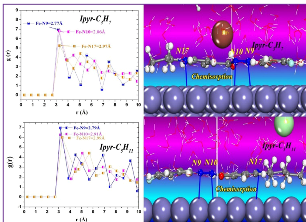
Fig. 18 RDF analysis of adsorbed Ipyr- \text{C}_3\text{H}_7 and Ipyr- \text{C}_5\text{H}_{11} on Fe(110) surface in a simulated acid medium at 298 K temperature obtained from MD simulation. [Reprinted with permission from ref. 104, ©2021 Elsevier.]
