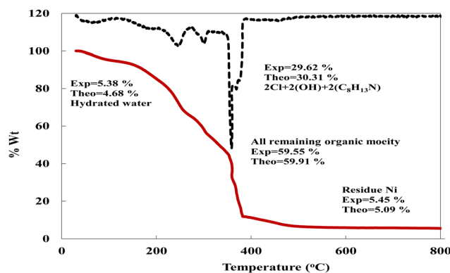
Fig. 3 TG curve of the prepared Ni(II)-SB complex.
