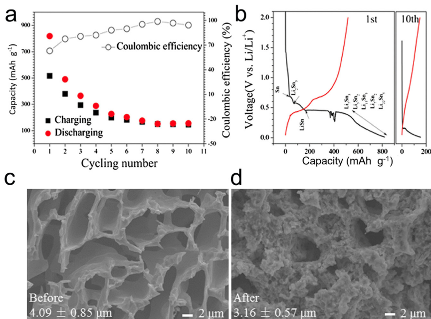
Fig. 14 (a) Cycling performance and (b) charge/discharge curve of the porous Sn dealloyed from Al_{60}Sn_{20} ; SEM images of the porous Sn structure before (c) and after (d) the lithiation/delithiation process. Reprinted with permission from ref. 127. Copyright 2015, Springer.
