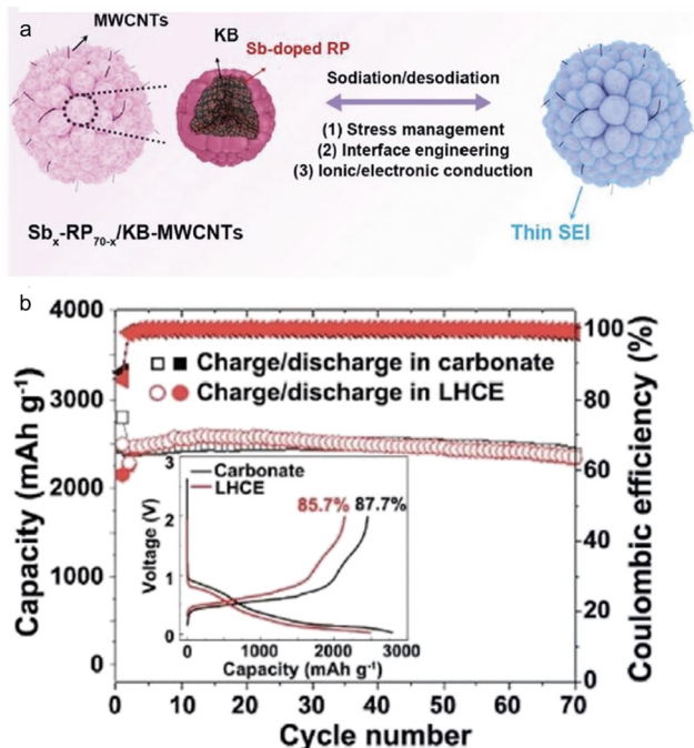
Fig. 13 (a) Schematic illustration and (b) cycling performance in carbonate electrolyte and localized highly concentrated ether electrolyte (LHCE) of hierarchical micro/nanostructured Sb_x-RP_{70-x}/KB-MWCNTs . Inset: first charge/discharge curve in two electrolytes. Reprinted with permission from ref. 125. Copyright 2021, American Chemical Society.
