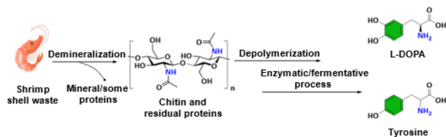
Fig. 10 Conversion of shrimp shell waste-derived chitin into aromatic amino acids. 26
