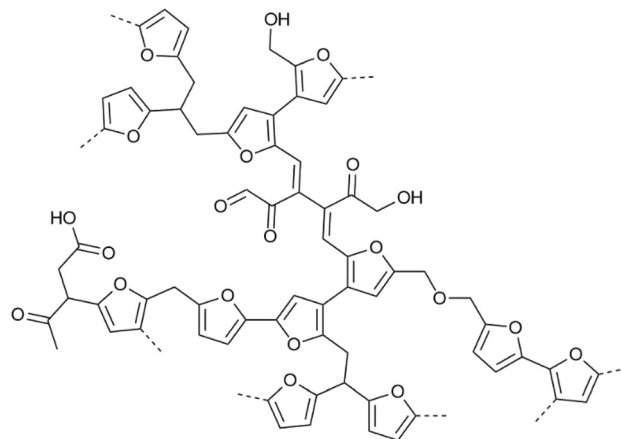
Fig. 1 Model for the molecular structure of a synthetic glucose-derived humin material. 37
